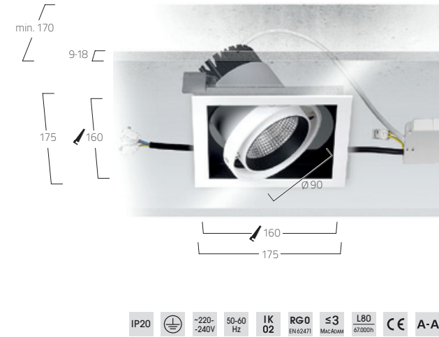
SPOT 10° LED ENGINE ECO, MEDIUM POWER
