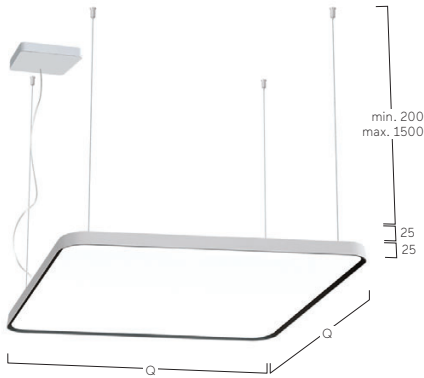
Parallel Suspension
