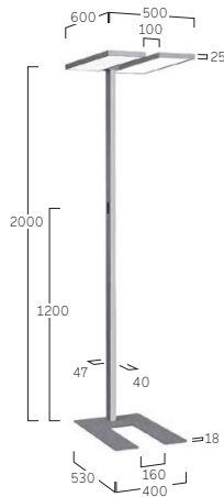
F6 Asymmetrical Stand, U- Cut-out
