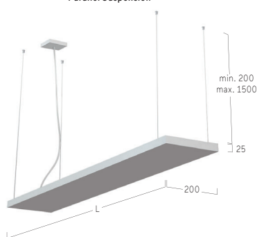
Parallel Suspension
