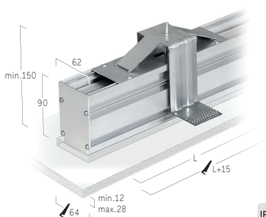
Installation Housing with Shadow Gap
