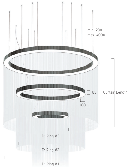
Parallel Suspension
