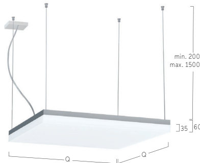
Parallel Suspension
