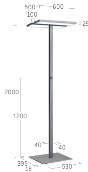
F5 Symmetrical Stand, Rectangular Base
