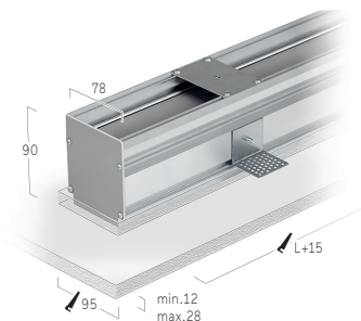
F: Installation Housing with Shadow Gap
