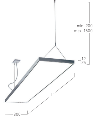
Y-Cord Suspension:
