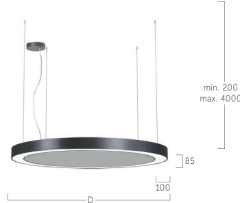
Parallel Suspension
