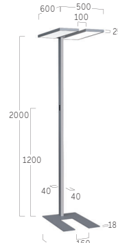
F6 Asymmetrical Stand, U- Cut Out
