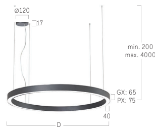
Parallel Suspension
